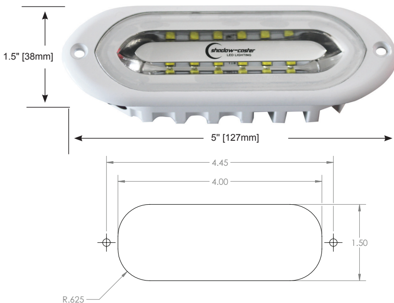
SCM-SLF-FLUSH MOUNT VERSION
